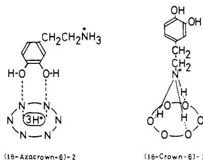
Figure 3. Proposed binding mode of dopamine (2) vs. 18-azacrown-6 (L) vs. 18-crown-6.
